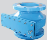
KSPC-KSFH Deflagration Flame Arrestor
